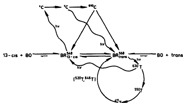
Fig.2 Simplified reaction scheme of the photochemistry and of the dark reactions of 13- cis and trans BR. Products originating from BR 548 13- cis after absorption of light at moderate intensity are designated as C, products originating from BR 568 trans are called T. A superscript on the right indicates the wavelength maximum of the absorption spectrum, a superscript on the left indicates the wavelength maximum of the difference absorption spectrum (spectrum of C product minus spectrum of 13- cis BR, spectrum of T product minus spectrum of trans BR). Superscripts x and y denote that the exact maxima of the difference spectra are presently unknown. The notation C and T does not say anything about the configuration of the chromophore of the transients (the reader is invited to compete for the correct subscript on the right).
