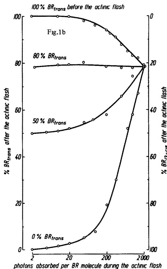
Fig 1 Isomeric composition of BR after exposure to light at different intensities Temperature 20°C (a) Linear scale, (b) abscissa logarithmic scale
